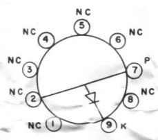
9 PIN NOVAR BASE
